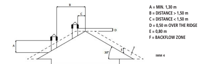
30° ROOF
