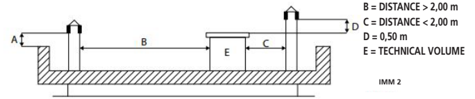
FLAT ROOF
