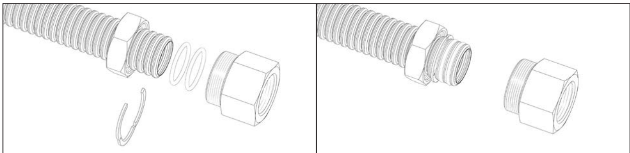
Figure 6.5.2 Pipe connection C-Clip
