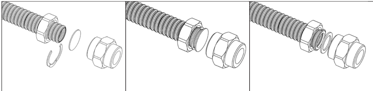
Figure 6.5.1 Corrugated pipe connection DN25
