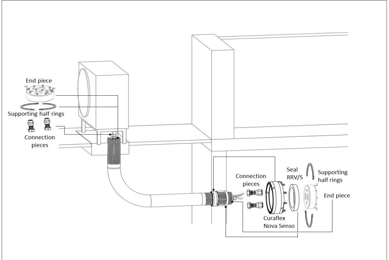
Figure 3.2 Basement lead-through type
