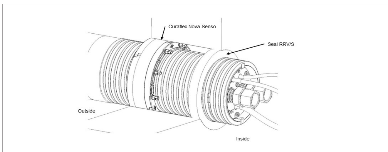
Figure 6.3.2 Seals for basement lead-through type
