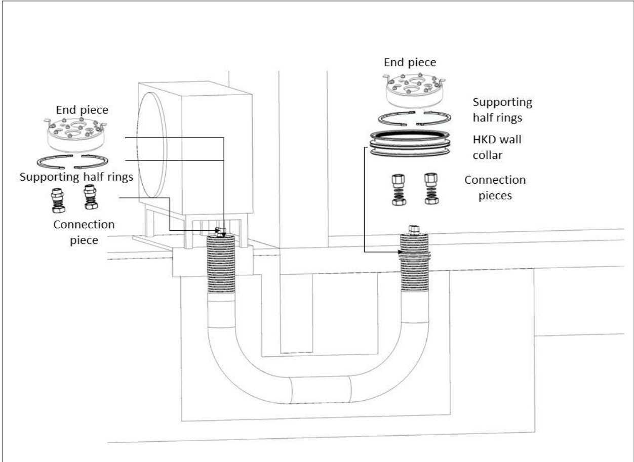
Figure 3.3 Base plate lead-through type
