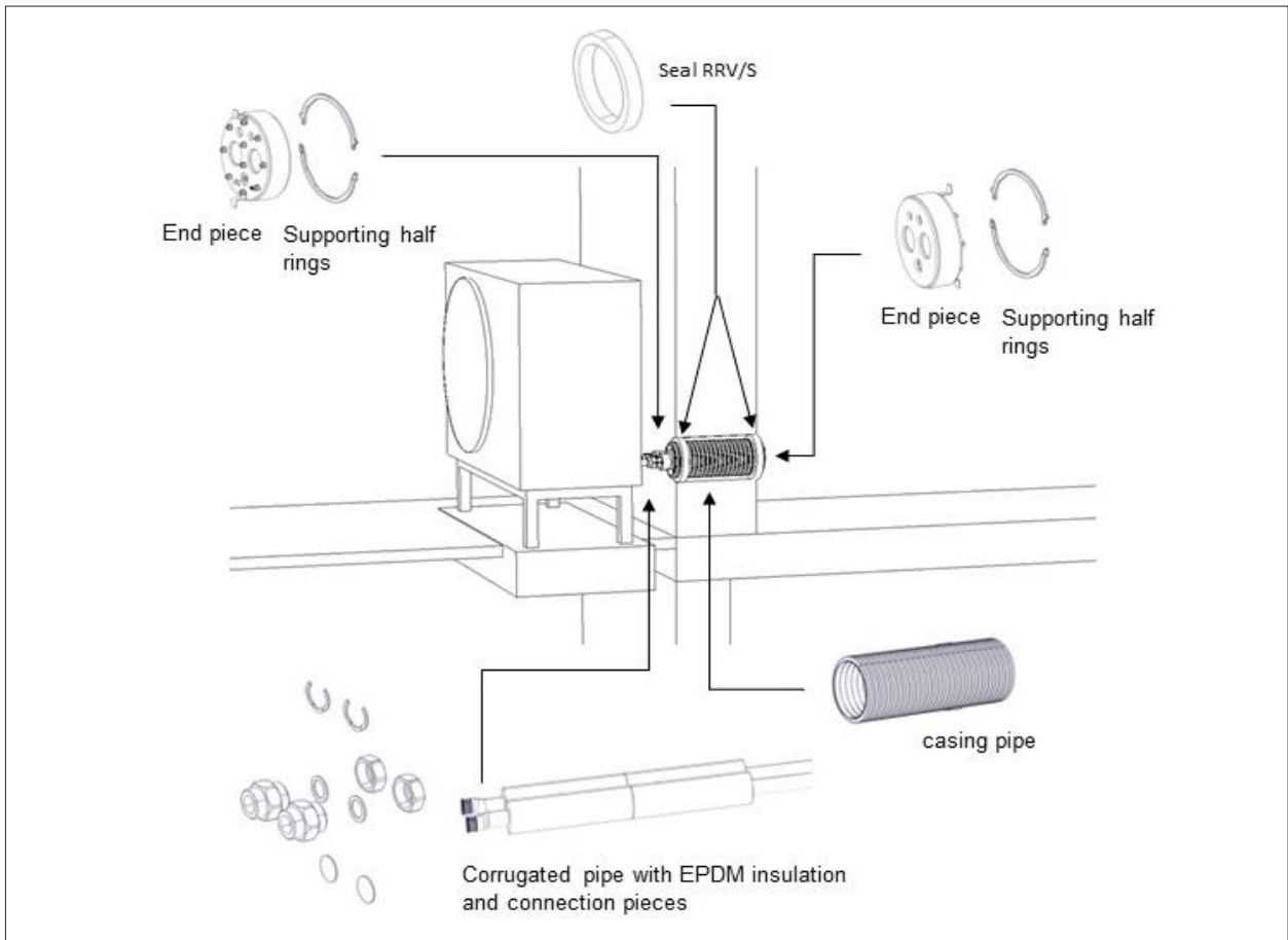
Figure 3.1 Facade lead-through type
