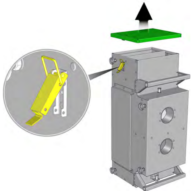
Abb. 4-2: Deckel
