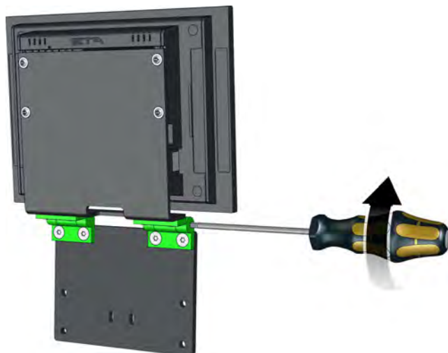
Abb. 2-5: Scharniere
