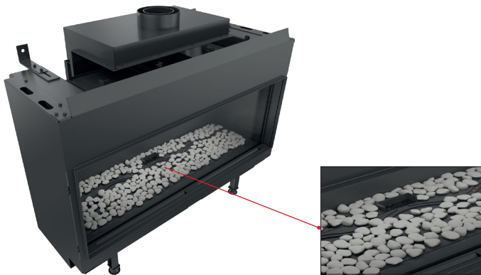
Figure 17. Proper distribution of decorative elements - stones
