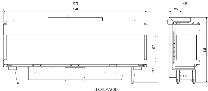
Rys. 2. Dimensions of the LEO 100 / LEO 200 gas inserts
