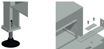
Figure 3. Levelling foot and adjustable bracket to attach to the wall
