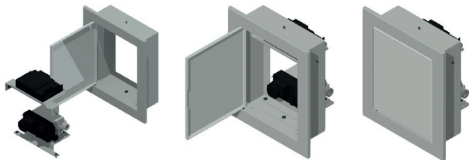
Figure 6. Mounting the gas controller with the receiver in the connection box
